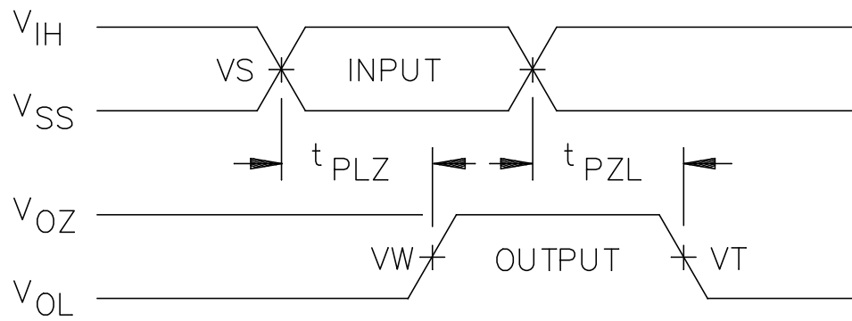
Three-state low timing diagram
