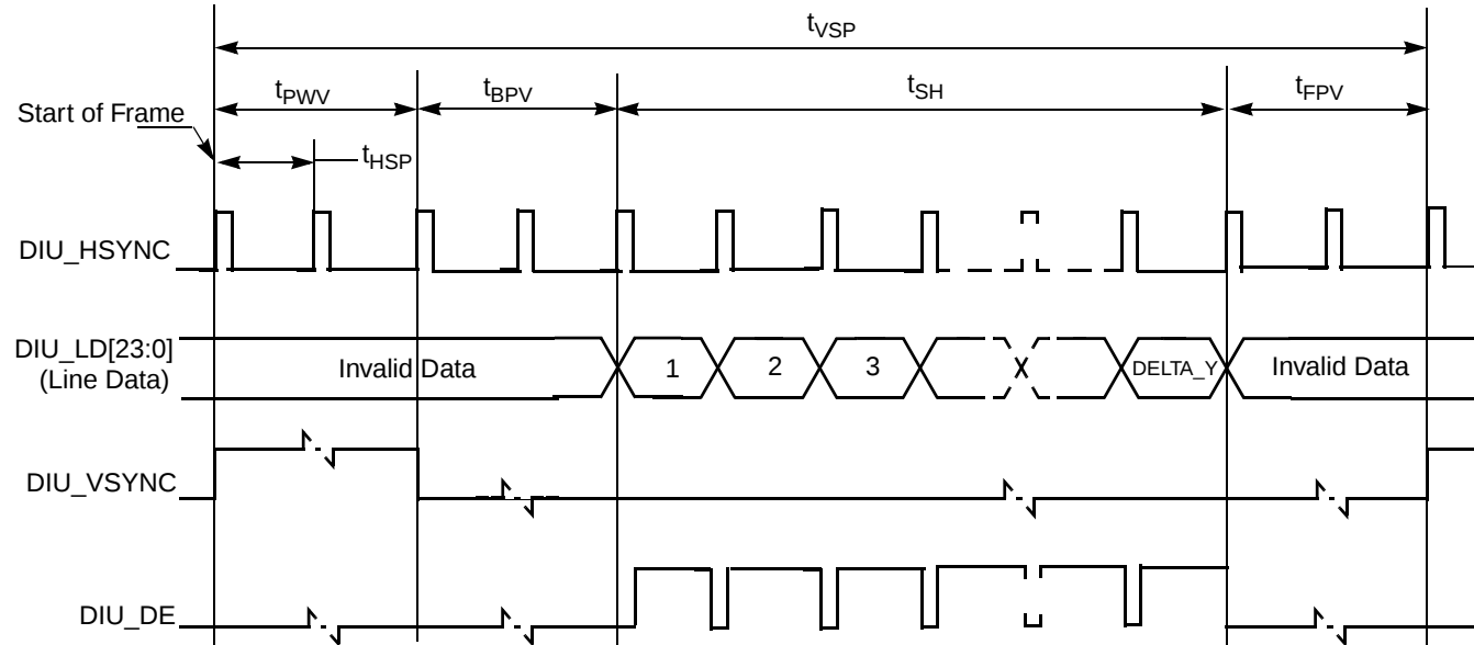
Figure 35. TFT LCD Interface Timing Diagram — Vertical Sync Pulse
