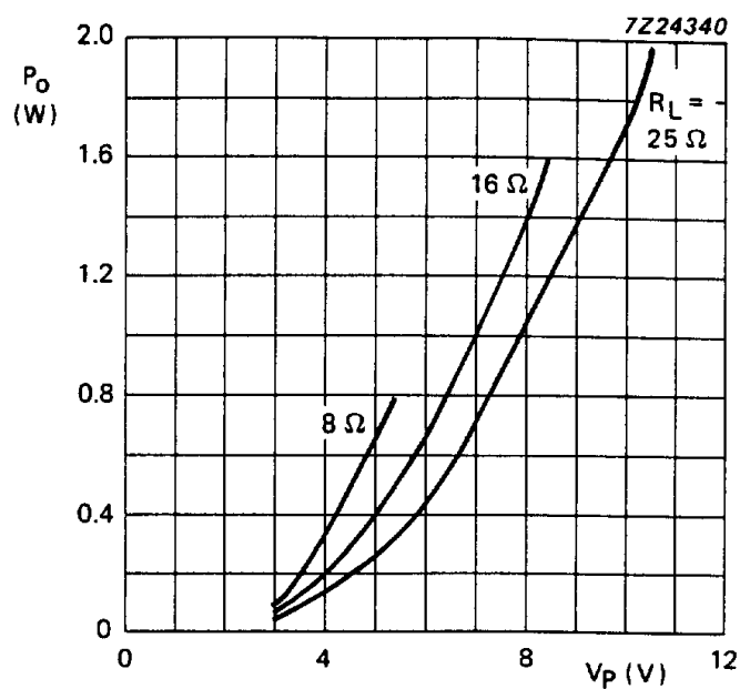
Fig.4 Output power as a function of voltage supply ( V_P ); THD = 10%; f = 1\ \text{kHz} ; T_{\text{amb}} = 60^\circ\text{C} .
