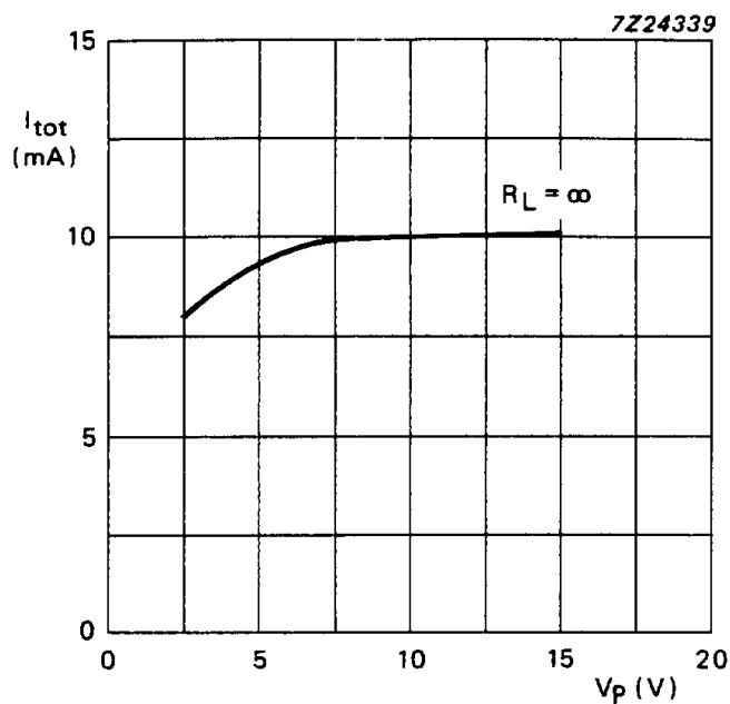
Fig.3 Quiescent current as a function of voltage supply ( V_P ); T_{\text{amb}} = 60^\circ\text{C} .
