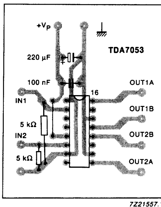
Fig.9 Printed-circuit board, component side.
