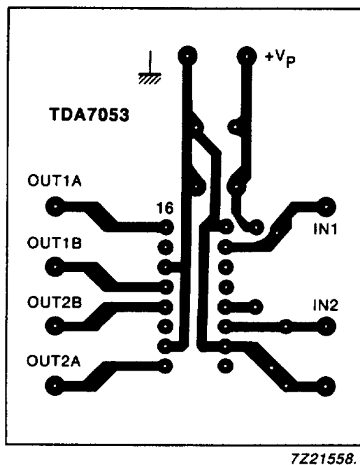
Fig.8 Printed-circuit board, track side.
