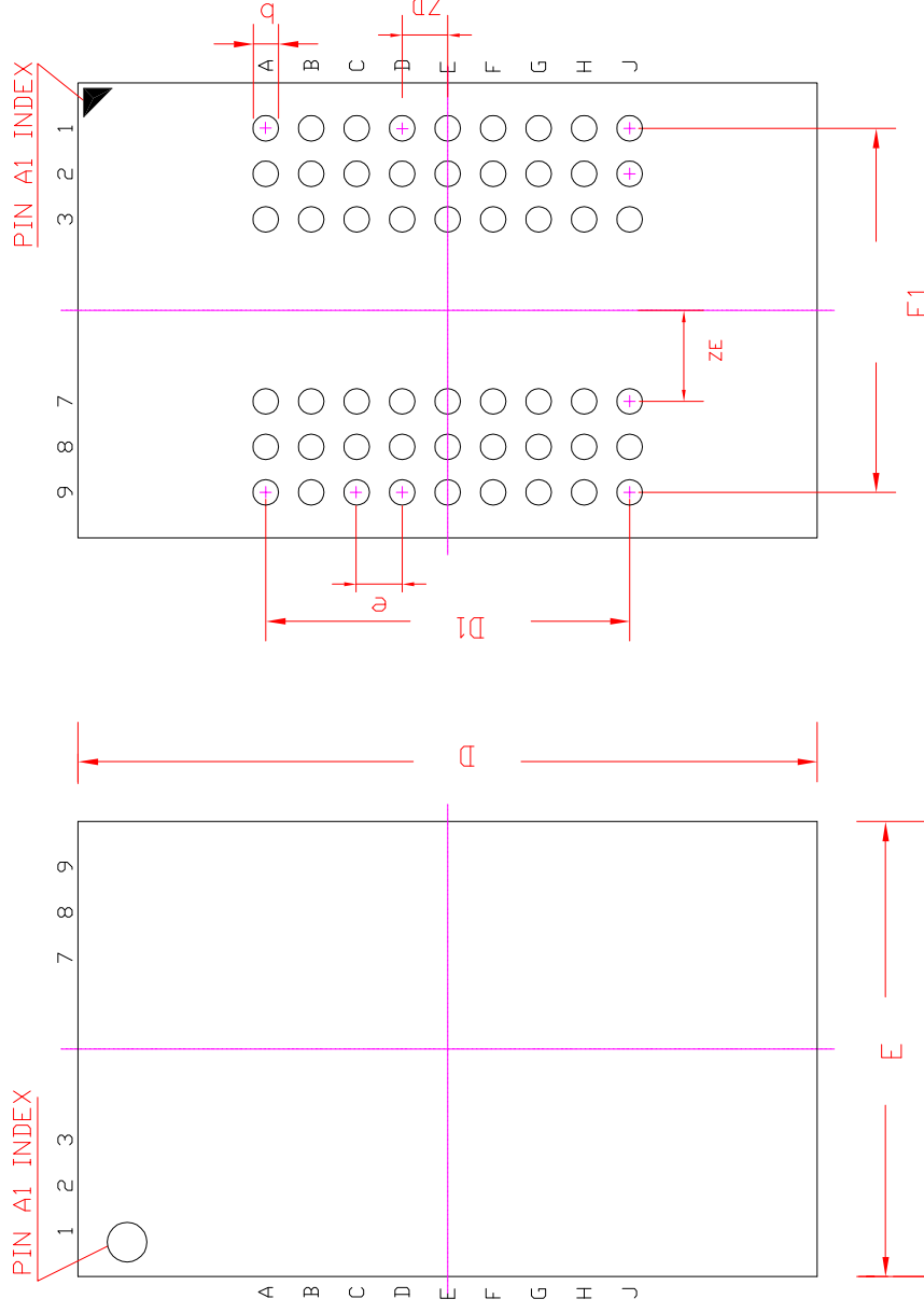
TOP VIEW
