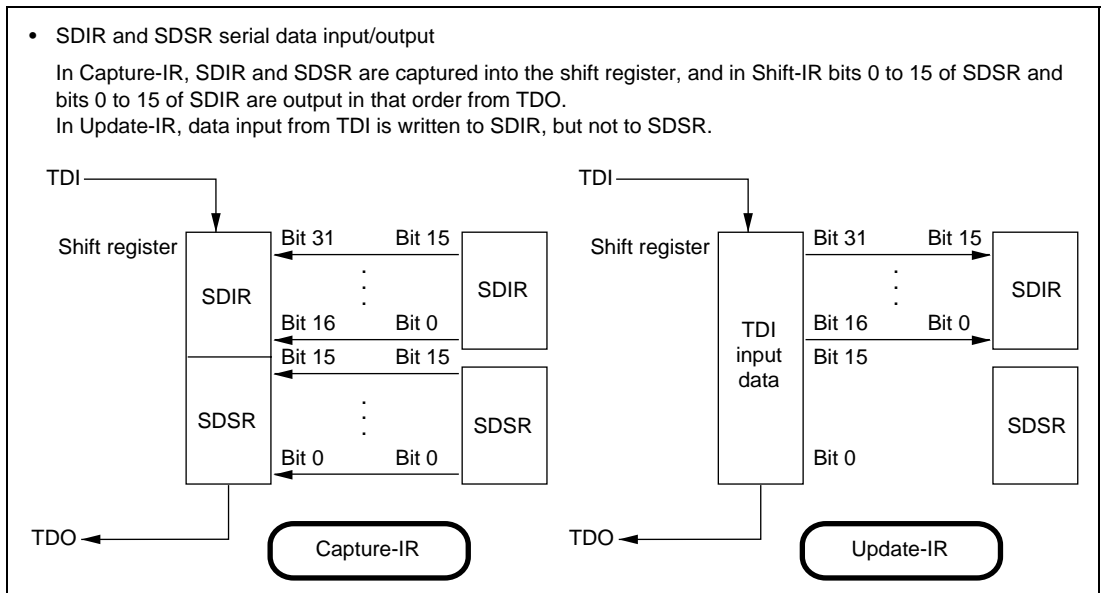
Figure 19.6 Serial Data Input/Output (1)
