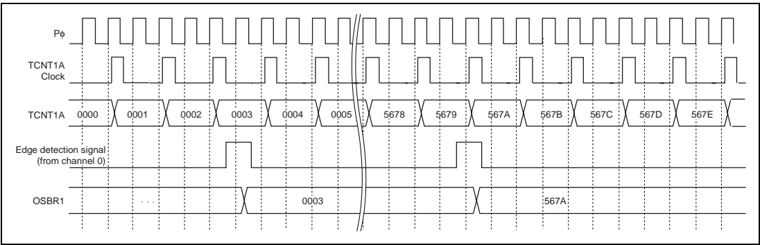
Figure 11.20 Twin-Capture Operation
