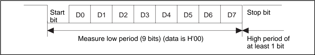
Figure 23.7 Automatic Adjustment Operation of SCI Bit Rate
