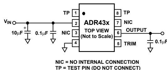
Figure 30. Basic Voltage Reference Configuration
