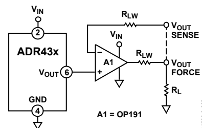
Figure 35. Advantage of Kelvin Connection
