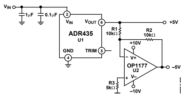
Figure 36. +5 V and -5 V References Using ADR435
