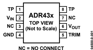
Figure 1. 8-Lead MSOP (RM Suffix)
