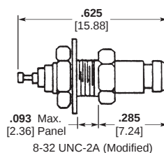
8-32 UNC-2A (Modified)
