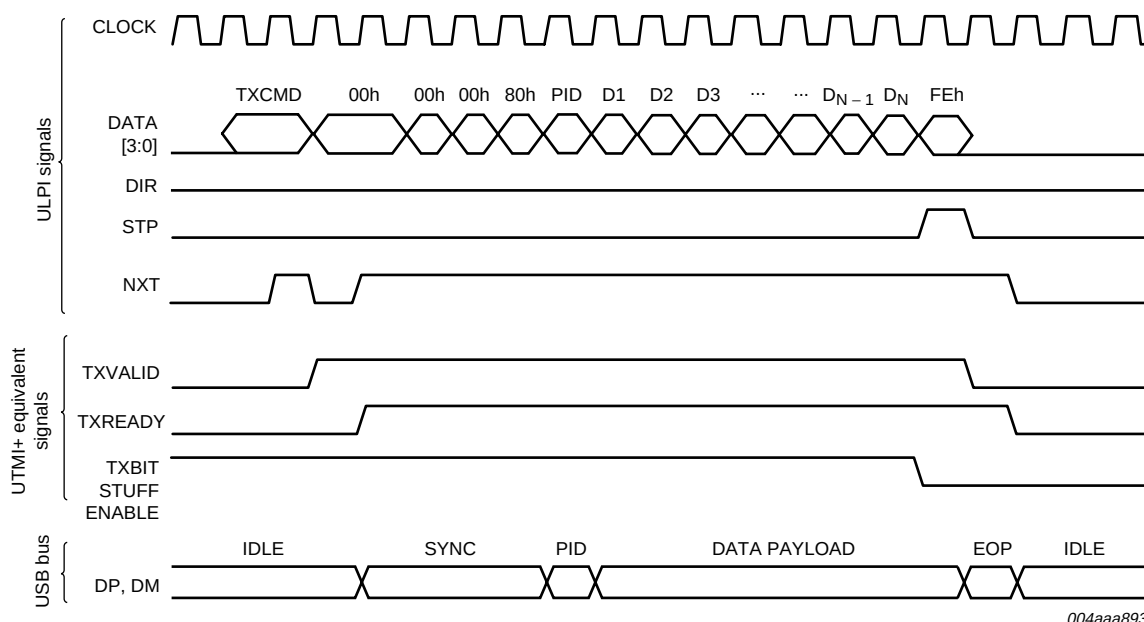
Fig 19. Transmitting USB packets without the automatic SYNC and EOP generation
