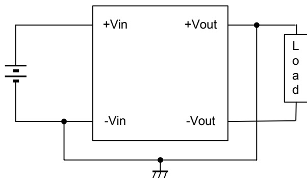
Connection to use turn around output voltage
