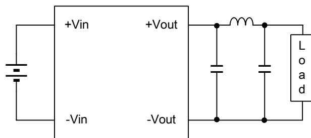
Connection to reduce output ripple voltage
