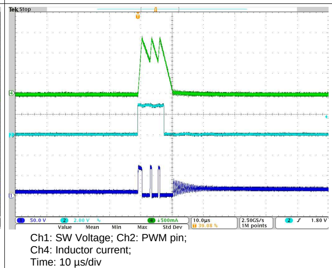
Figure 39. PWM Dimming: 250Hz, 0.25% Duty Cycle
