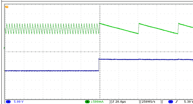
Ch1: PWM Signal Ch4: Inductor current; \Delta I_{L-PP} Maintained Time: 20 \mu s/div
