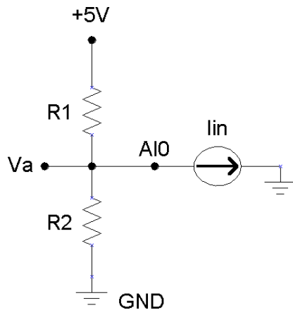
Figure 2-4. Single-ended measurement with voltage divider circuit.
