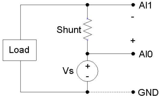
Figure 2-3. Differential measurement.
