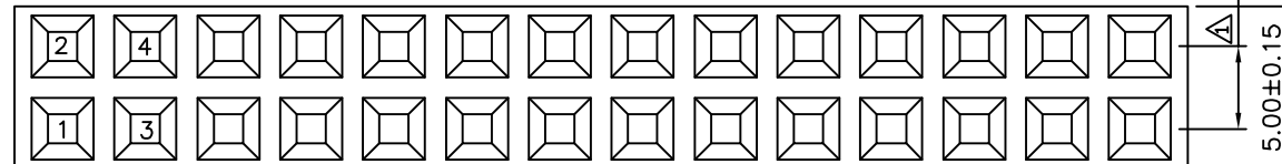
△ Recommended P.C.B. Layout(Top Side) (PCB Board Tolerance \pm 0.05 )
