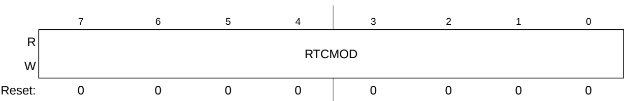
Figure 14-5. RTC Modulo Register (RTCMOD)
