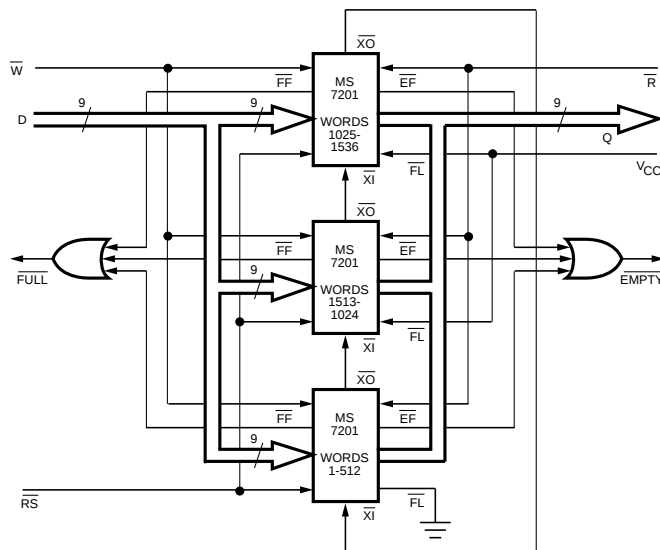
Figure 5. Diagram of a 1536 x 9 FIFO in Depth Expansion Mode
