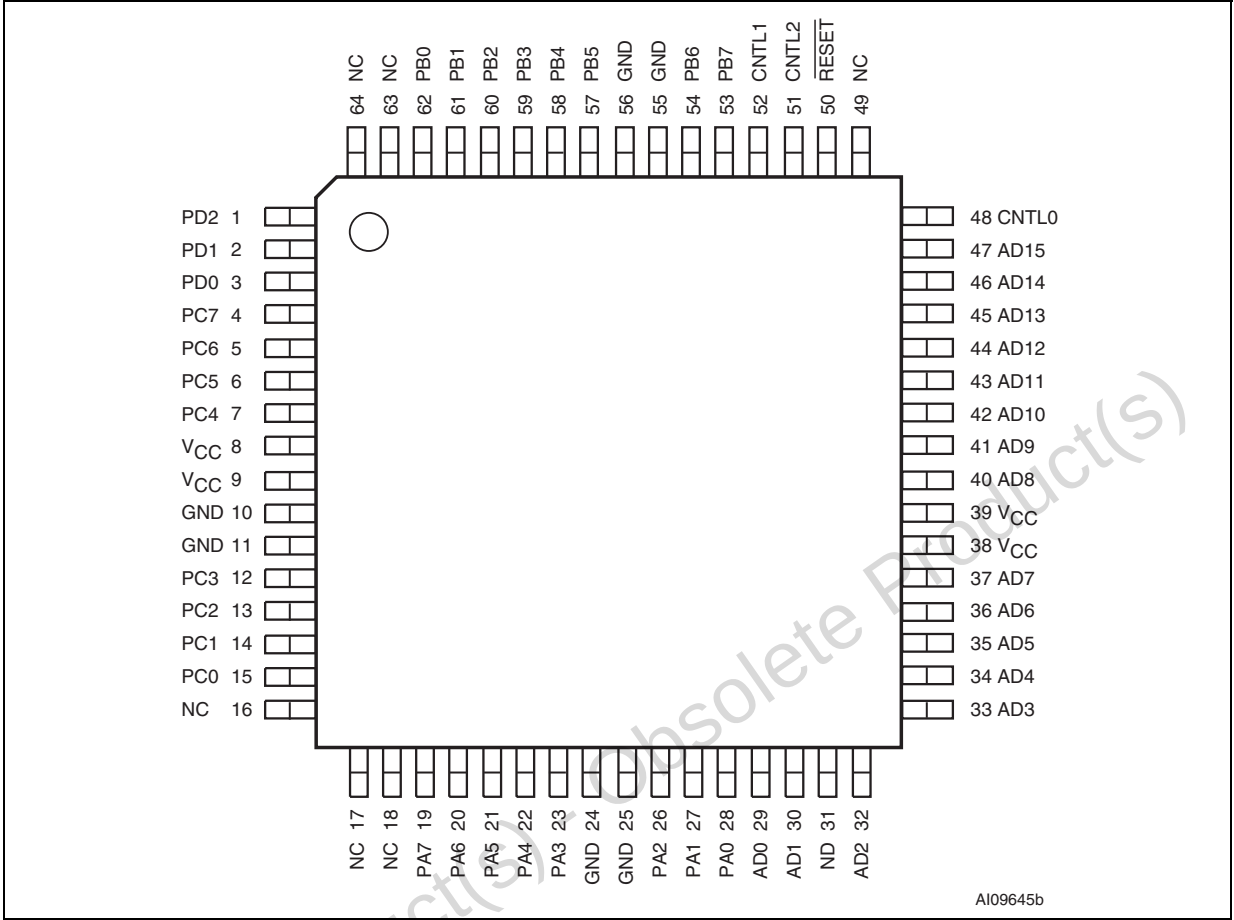
Figure 3. TQFP64 connections
