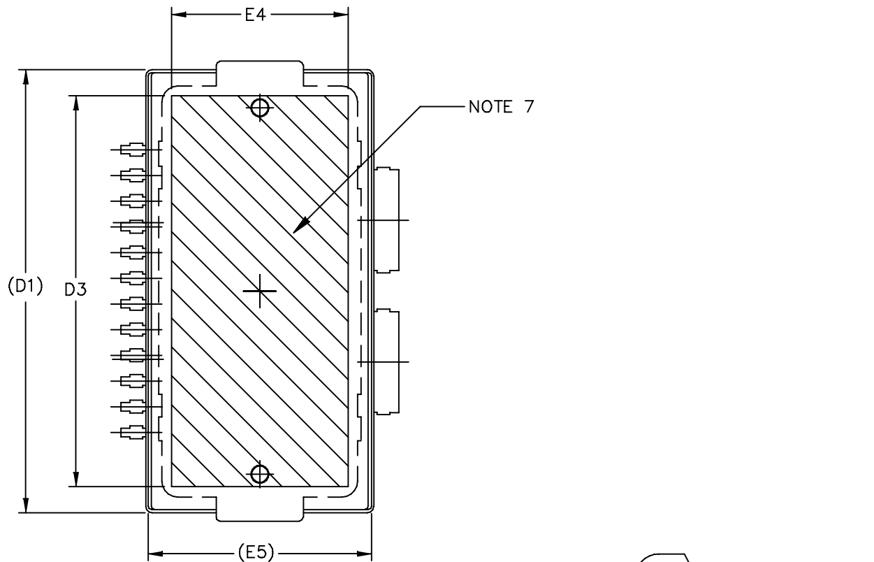
VIEW Y-Y
