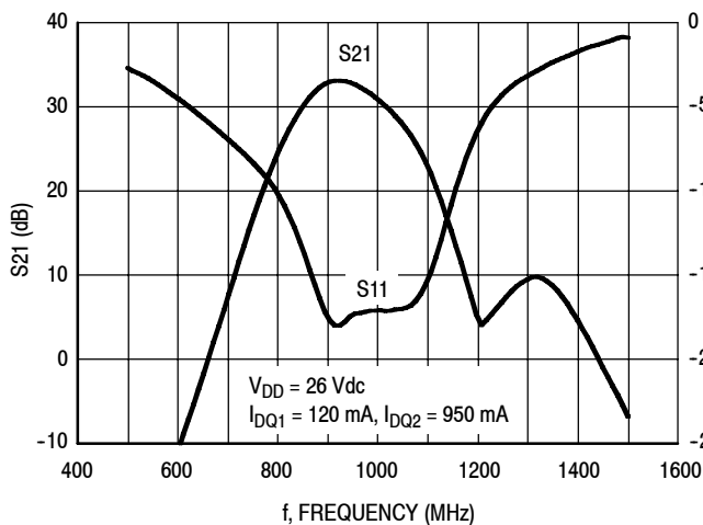
Figure 23. Broadband Frequency Response
