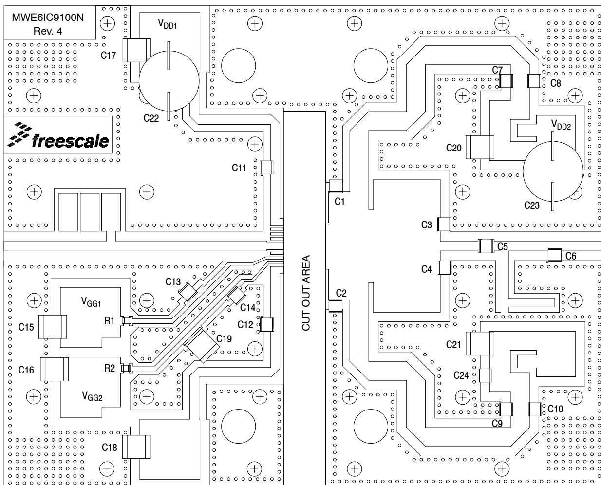
Figure 4. MWE6IC9100NR1(GNR1)(NBR1) Test Circuit Component Layout
