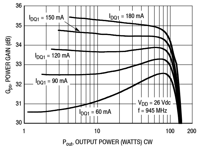
Figure 8. Power Gain versus Output Power @ I_{DQ2} = 950 mA
