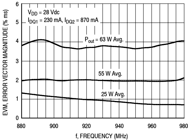
Figure 15. EVM versus Frequency
