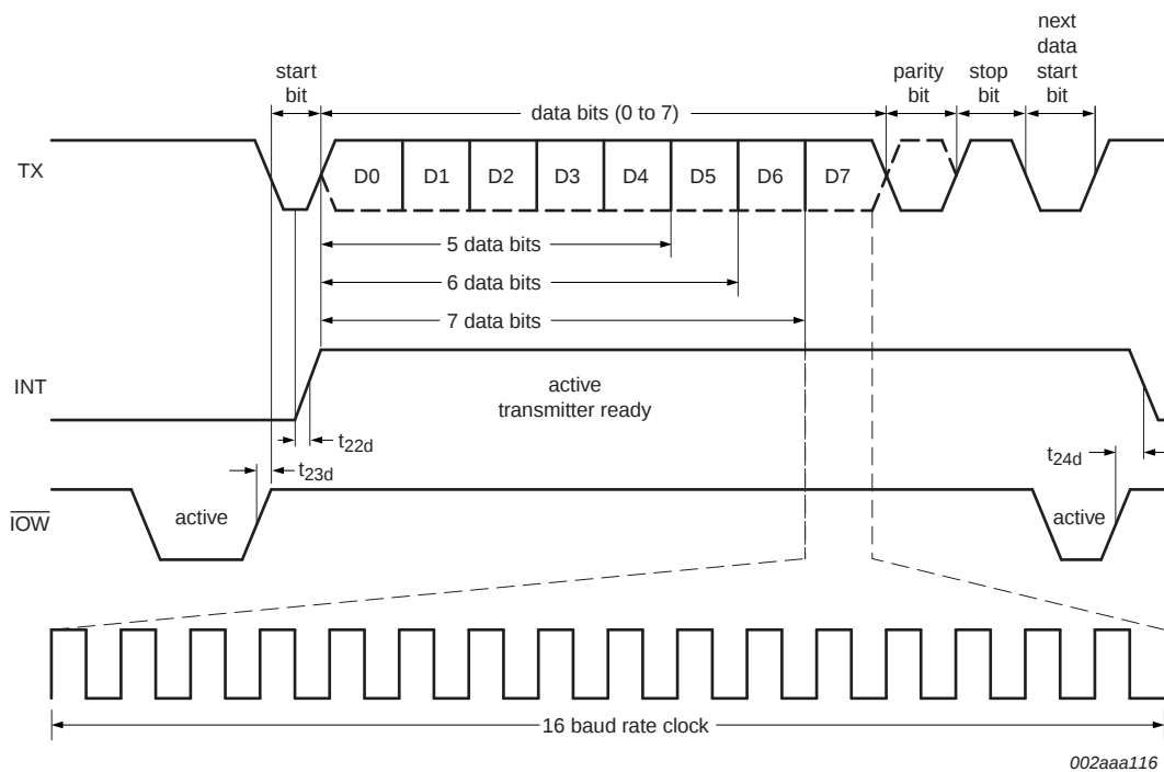
Fig 21. Transmit timing
