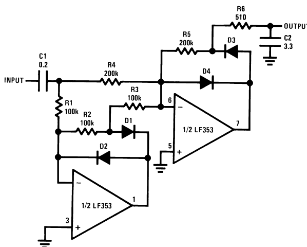
FIGURE 5. Precision Full-Wave Average Detector
