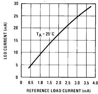
LED Current vs Referenced Loading
