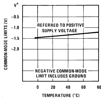
Common-Mode Limits
