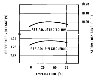
Reference Voltage vs Temperature
