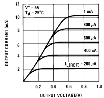
Output Characteristics
