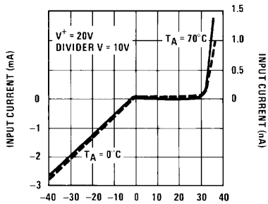
Input Current Beyond Signal Range (Pin 5)
