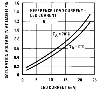
LED Driver Saturation Voltage
