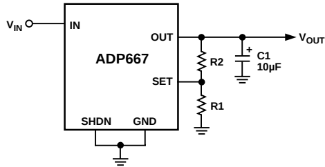
Figure 3. Adjustable Output Circuit
