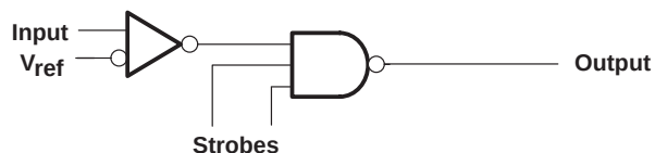
Figure 13. Single-Ended Operation
