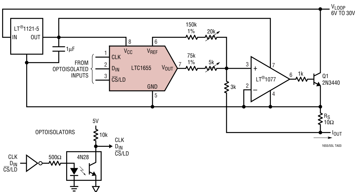
An Isolated 4mA to 20mA Process Controller
