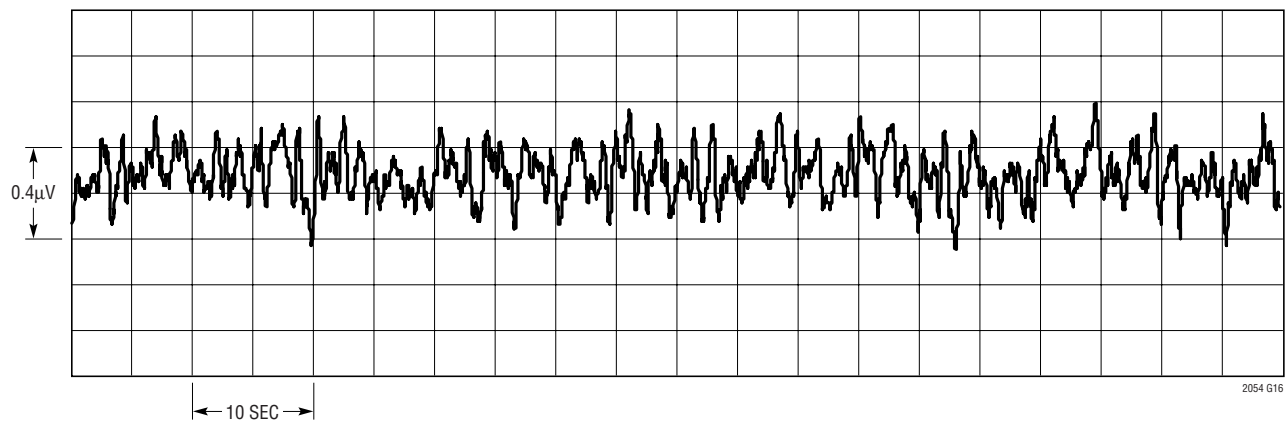
LTC2054 DC to 1Hz Noise
