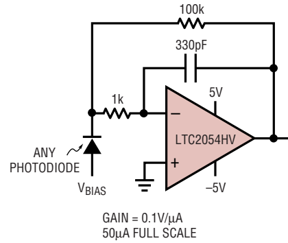
Ultra-Precision, Wide Dynamic Range Photodiode Amplifier
