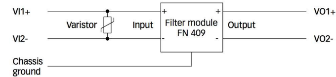
Figure 1: transient protection with a varistor
