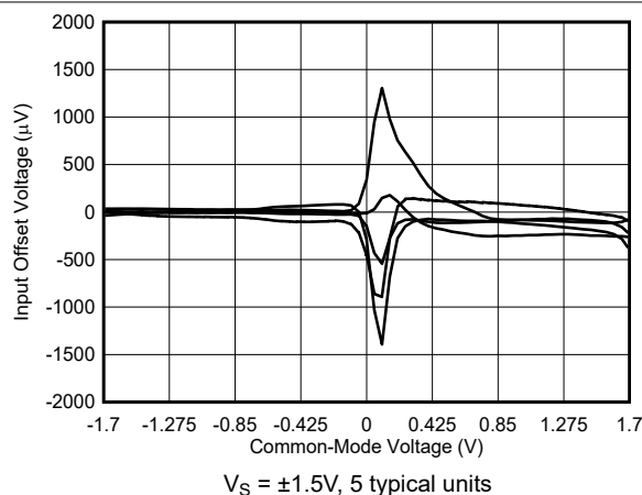
Figure 6-10. Input Offset Voltage vs Common-Mode Voltage
