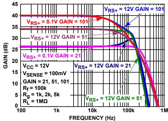
FIGURE 59. GAIN vs FREQUENCY V_{RS+} = 100mV/12V , V_{SENSE} = 100mV , V_{OUT} = 50mV_{P-P}
