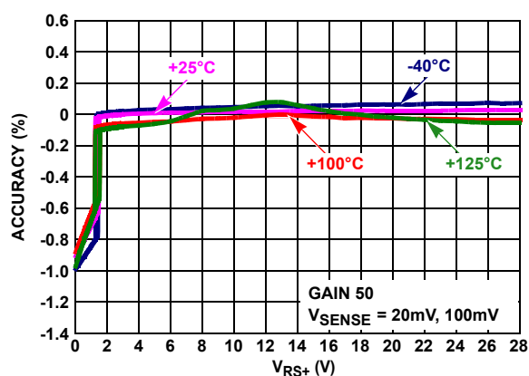
FIGURE 26. GAIN ACCURACY vs V_{RS+} = 0V TO 28V
