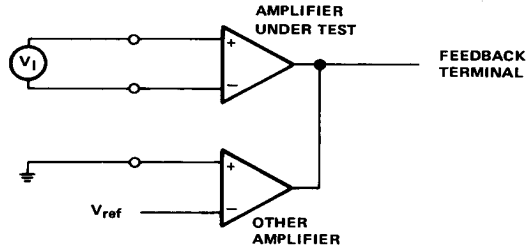
FIGURE 2. AMPLIFIER CHARACTERISTICS
