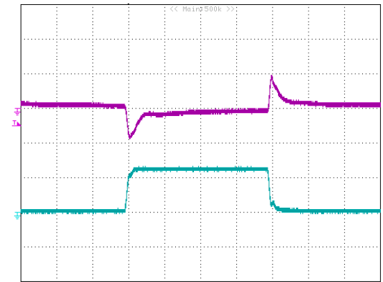
Figure 22: Typical transient response to step load change at 2.5A/\mu s from 0% to 50% to 0% of I_o , max at 5V_{in} , 3.3V_{out} (100uS/div) ( C_{out} = 47\mu F ceramic). top trace: V_{out} , 0.2V/div; bottom trace: I_{out} : 5A/div.
