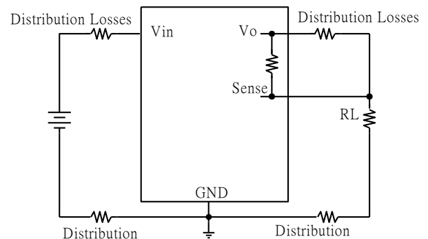
Figure 30: Effective circuit configuration for remote sense operation
