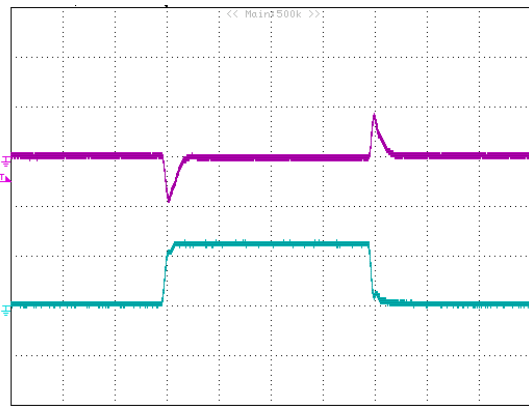
Figure 21: Typical transient response to step load change at 2.5A/\mu s from 0% to 50% to 0% of I_o , max at 5V_{in} , 1.8V_{out} (100uS/div) ( C_{out} = 47\mu F ceramic). top trace: V_{out} , 0.2V/div; bottom trace: I_{out} : 5A/div.
