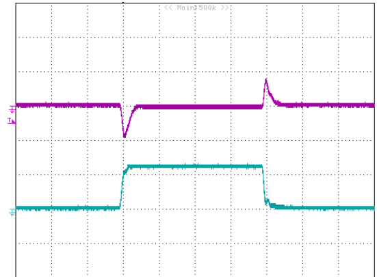
Figure 20: Typical transient response to step load change at 2.5A/\mu s from 0% to 50% to 0% of I_o , max at 5V_{in} , 1.2V_{out} (100uS/div) ( C_{out} = 47\mu F ceramic). top trace: V_{out} , 0.2V/div; bottom trace: I_{out} : 5A/div.
