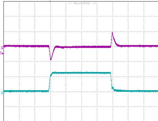
Figure 19: Typical transient response to step load change at 2.5A/\mu s from 0% to 50% to 0% of I_o , max at 5V_{in} , 0.6V_{out} (100uS/div) ( C_{out} = 47\mu F ceramic). top trace: V_{out} , 0.2V/div; bottom trace: I_{out} : 5A/div.
