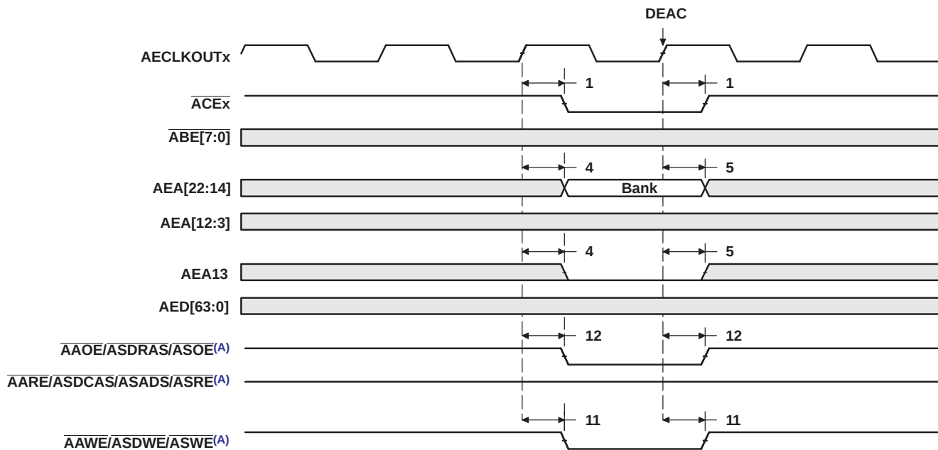
Figure 5-28. SDRAM DEAC Command for EMIFA
