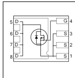
PQFN 3.3 X 3.3 mm
