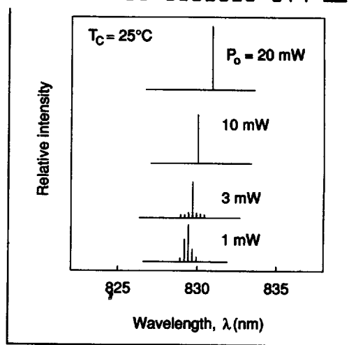
Figure 2 Lasing Spectrum
