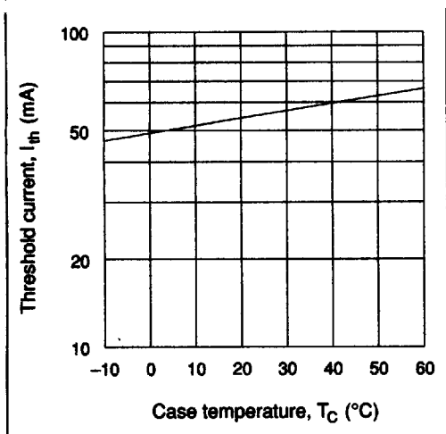
Figure 5 Temperature Dependence of Threshold Current
