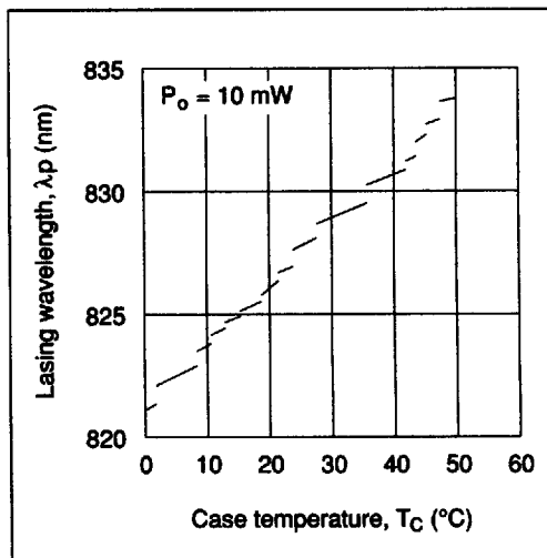
Figure 8 Temperature Dependence of Lasing Wavelength
