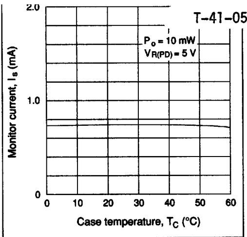
Figure 6 Temperature Dependence of Monitor Current
