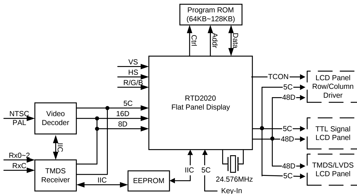
Application System Block Diagram
