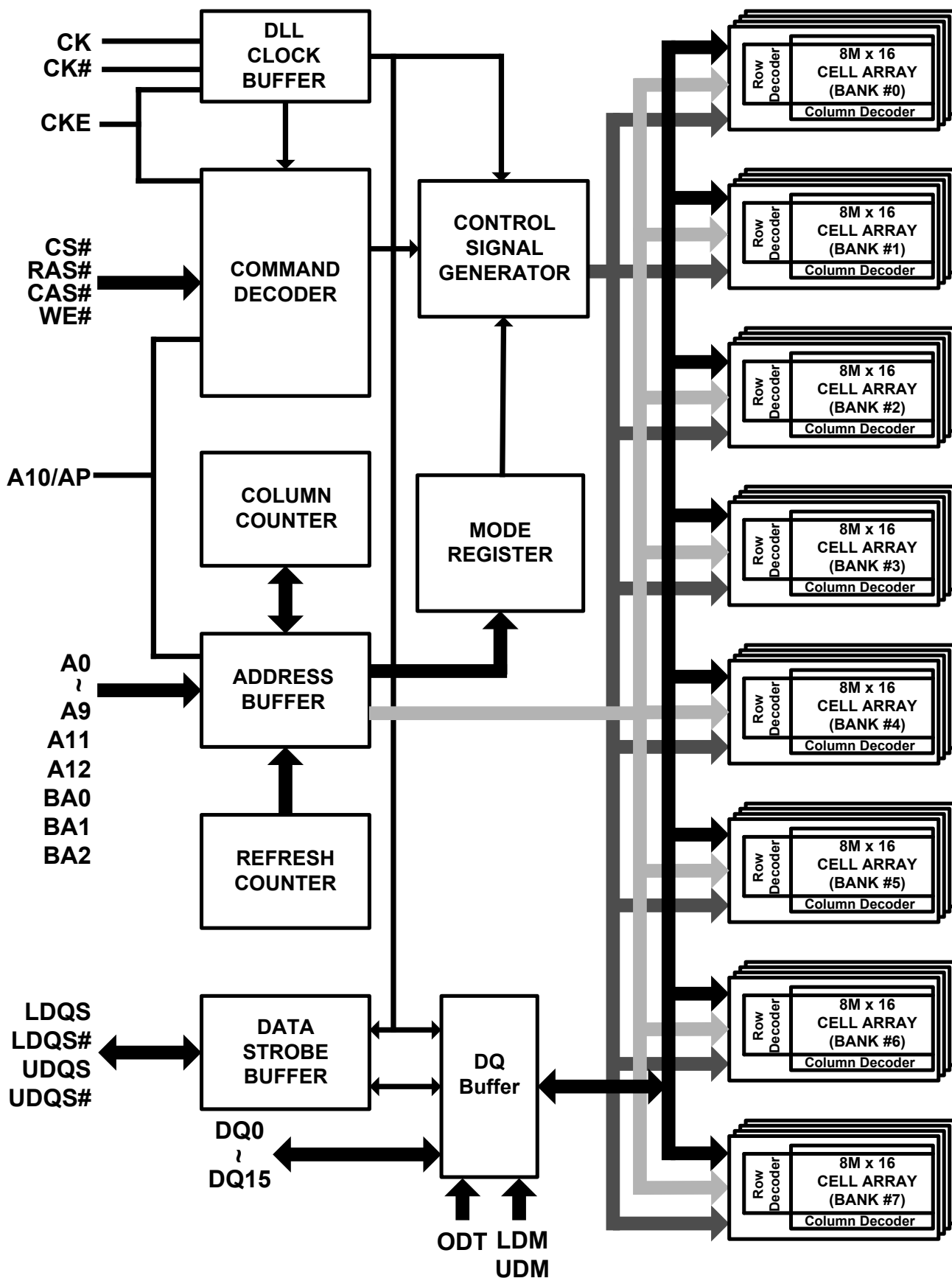
Figure 2. Block Diagram
