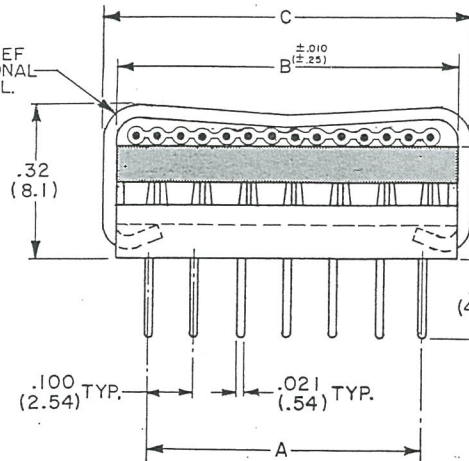
CONNECTOR COVER SHOWN IN OPEN POSITION
