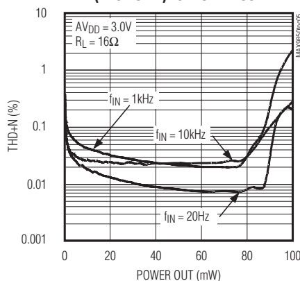
TOTAL HARMONIC DISTORTION PLUS NOISE (LINE IN TO HP) vs. POWER OUT
