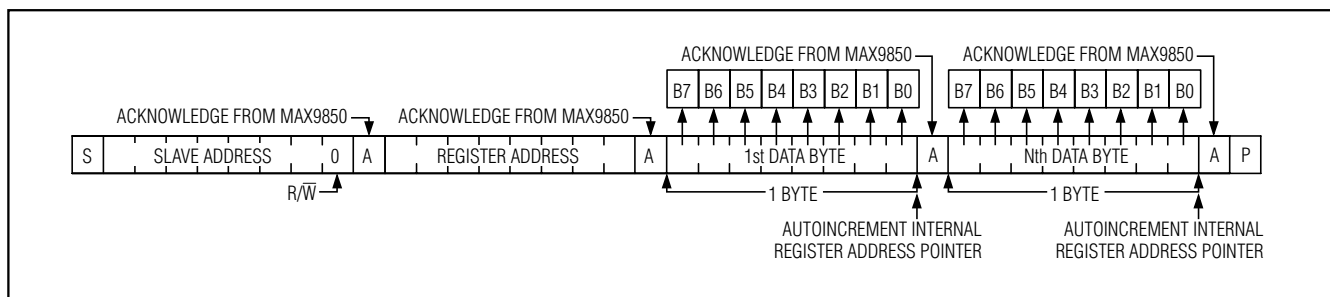
Figure 9. Writing n-Bytes of Data to the MAX9850
