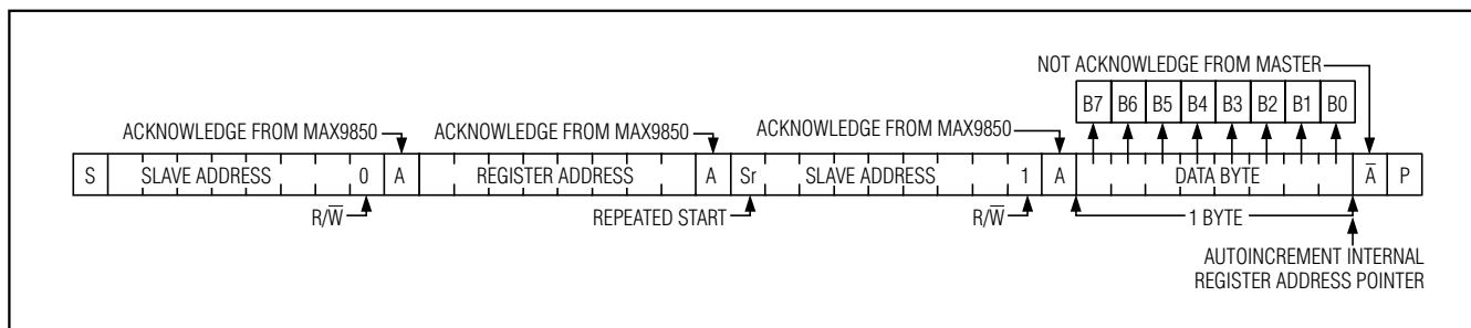
Figure 10. Reading One Byte of Data from MAX9850
