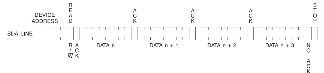
Figure 6. Sequential Read
