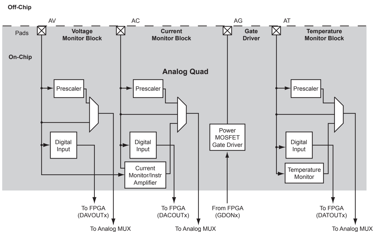
Figure 2-65 • Analog Quad
