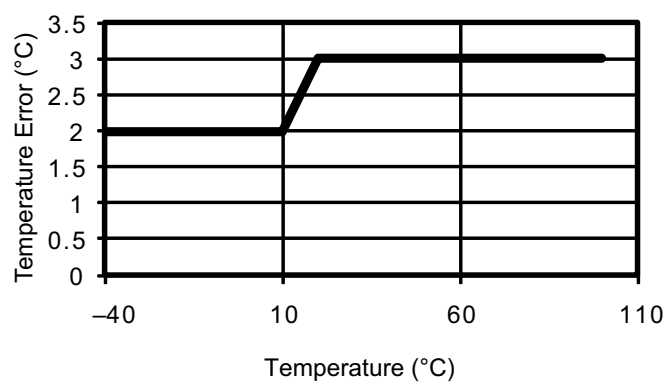
Figure 2-94 • Temperature Error
