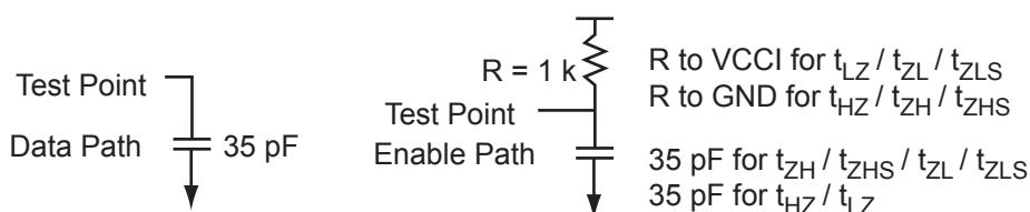
Figure 2-119 • AC Loading
