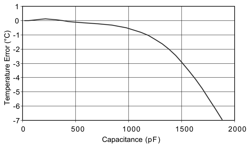
Figure 2-95 • Effect of External Sensor Capacitance
