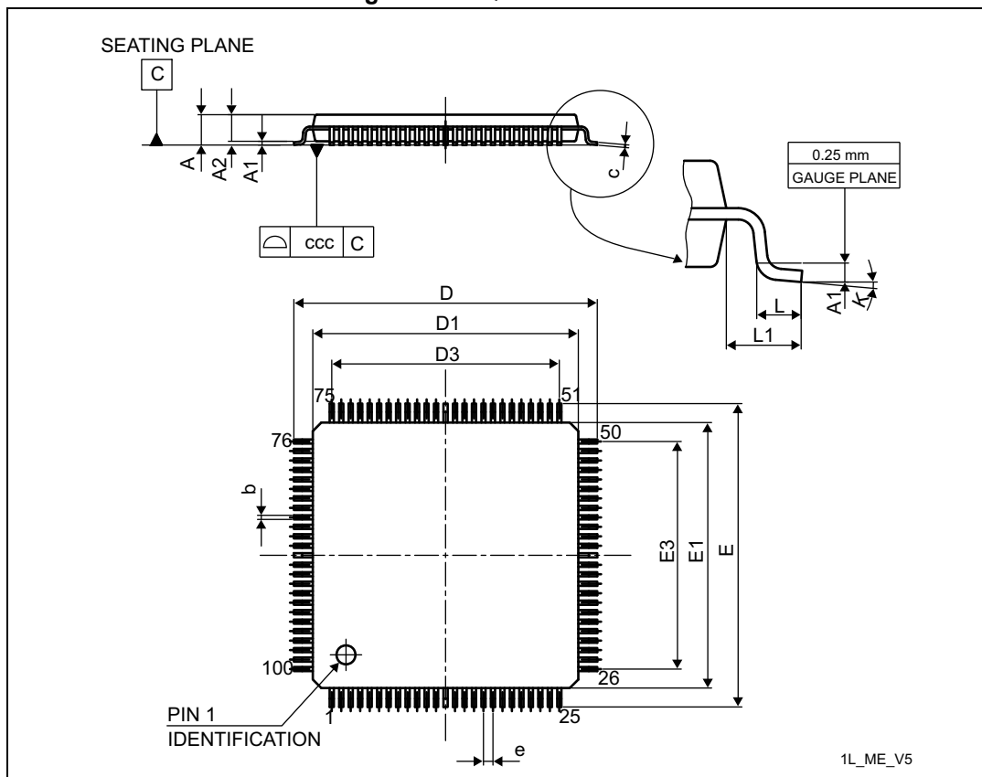
Figure 74. LQFP100 outline
