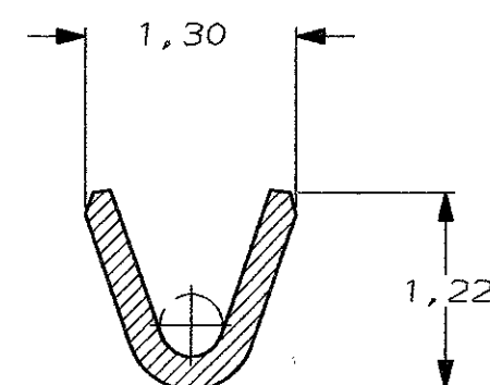
SECTION B-B SCALE 20:1
