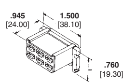
Receptacle Housing
