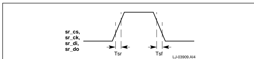
Figure 20. Serial ROM Port Timing Diagram
