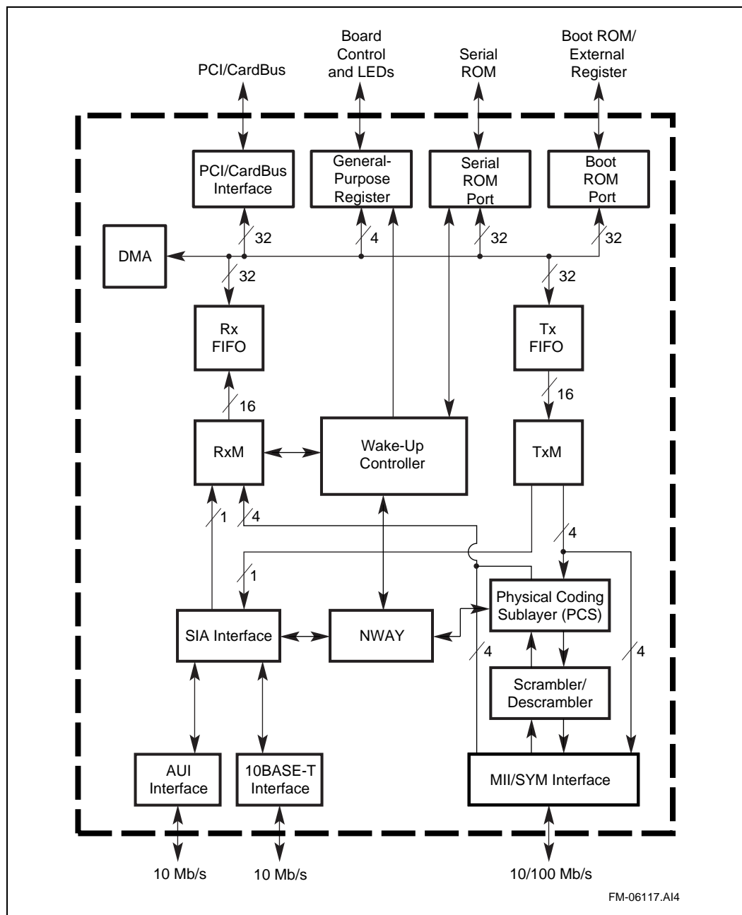
Figure 1. 21143 Block Diagram
