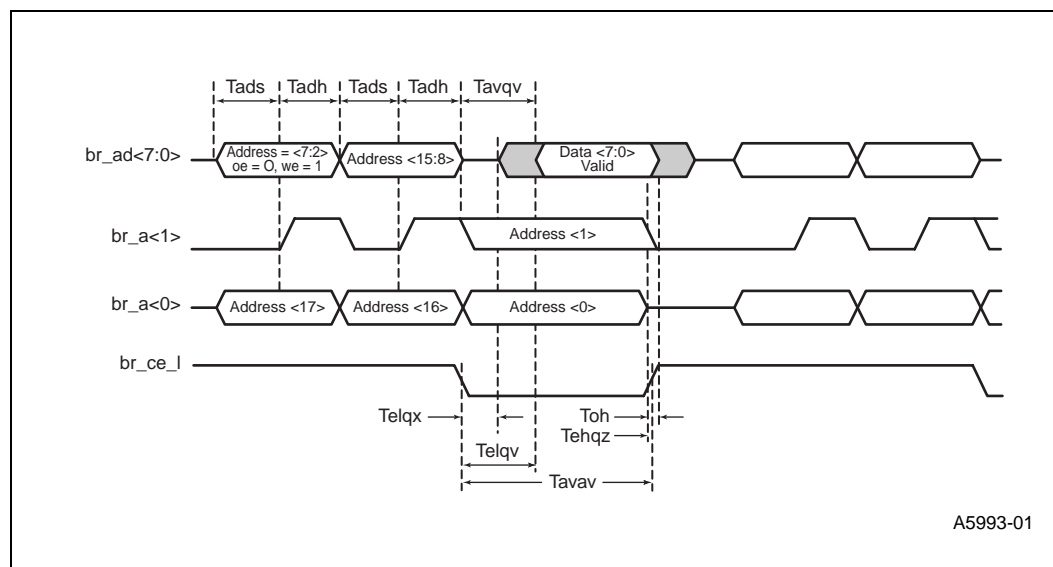
Figure 18. Boot ROM Read Timing Diagram
