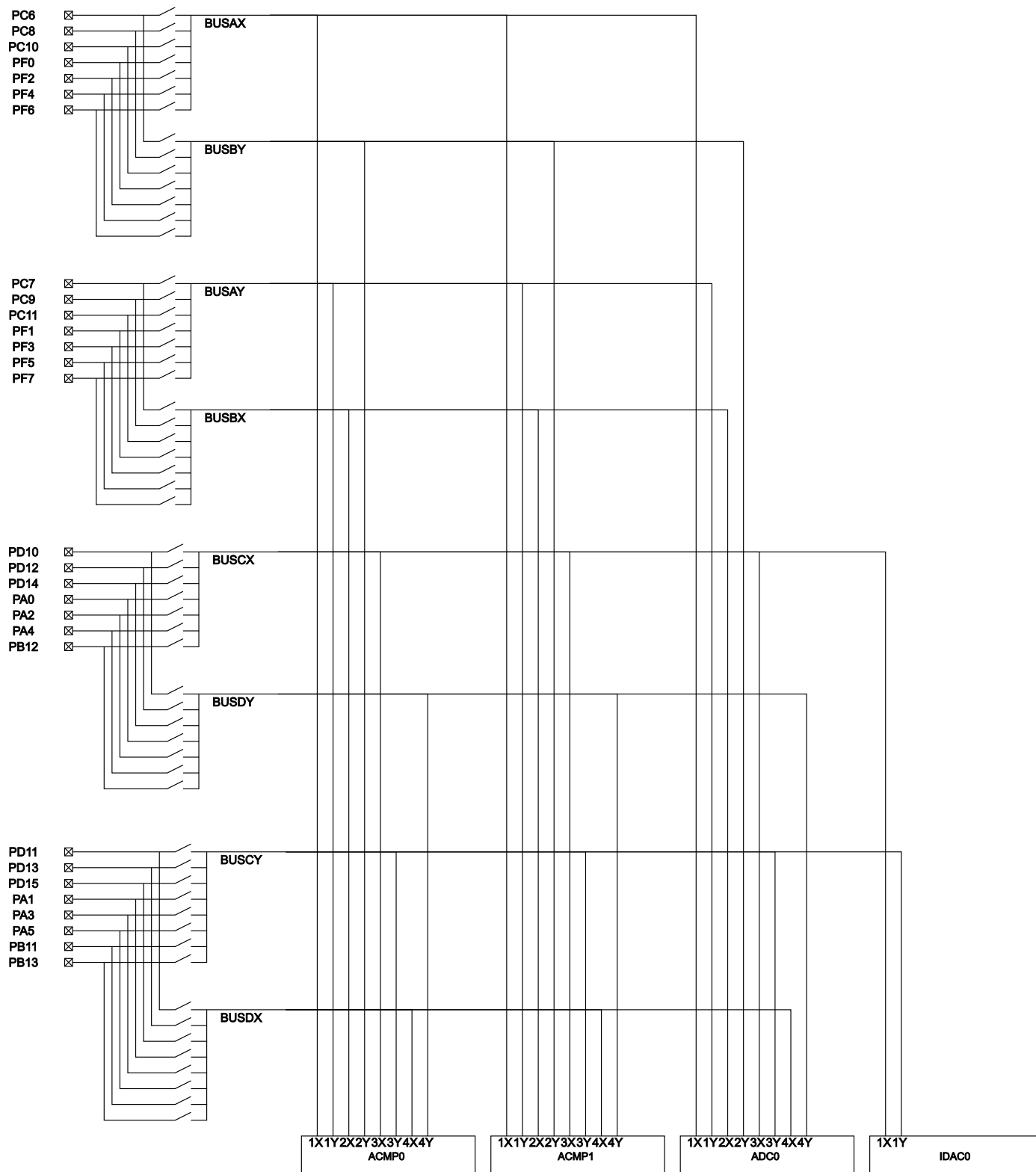
Figure 7.2. BGM121/BGM123 APORT
