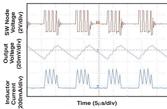
Figure 10. Power-Save Mode
