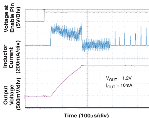
Figure 13. Start-Up Response
