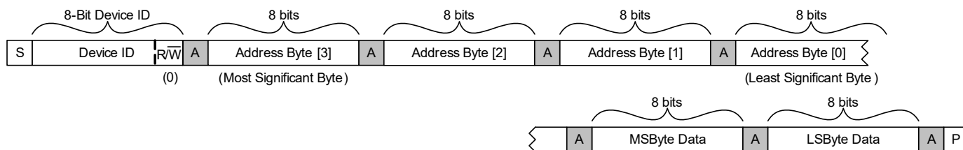
Figure 4-74. Single-Register Write to Specified Address
