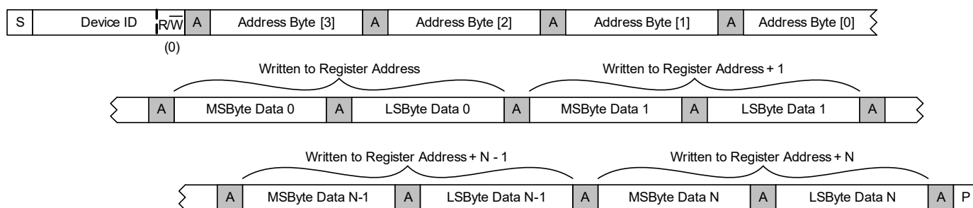
Figure 4-76. Multiple-Register Write to Specified Address
