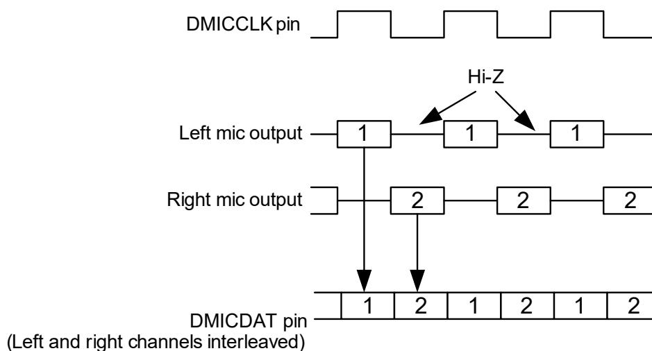
Figure 4-12. DMIC Interface Timing
