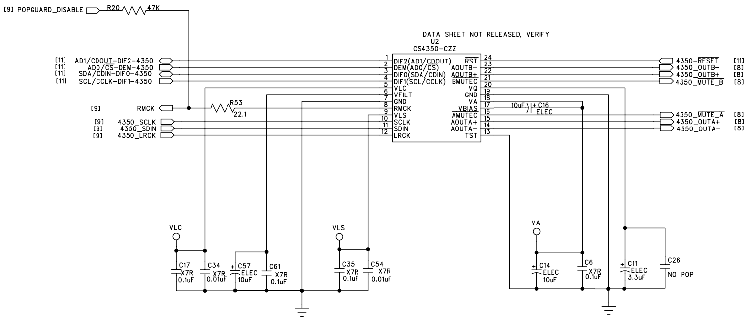
Figure 2. CS4350
