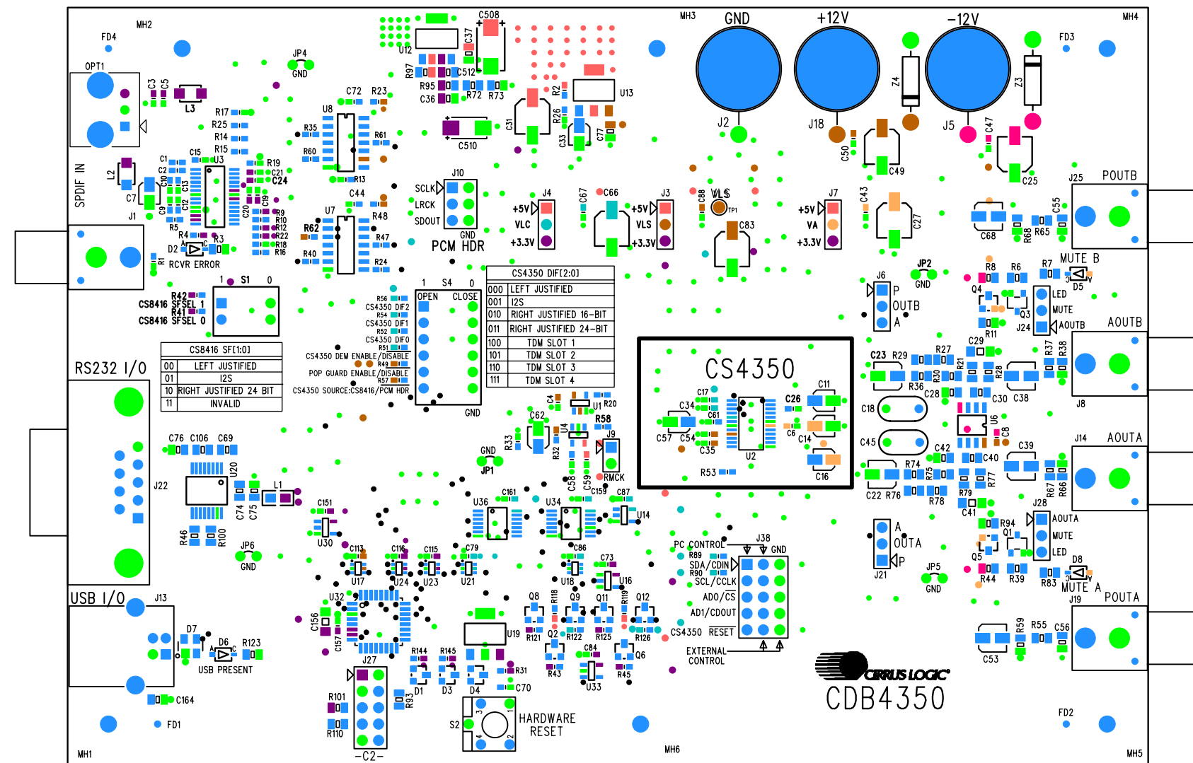
Figure 8. Silkscreen Top
