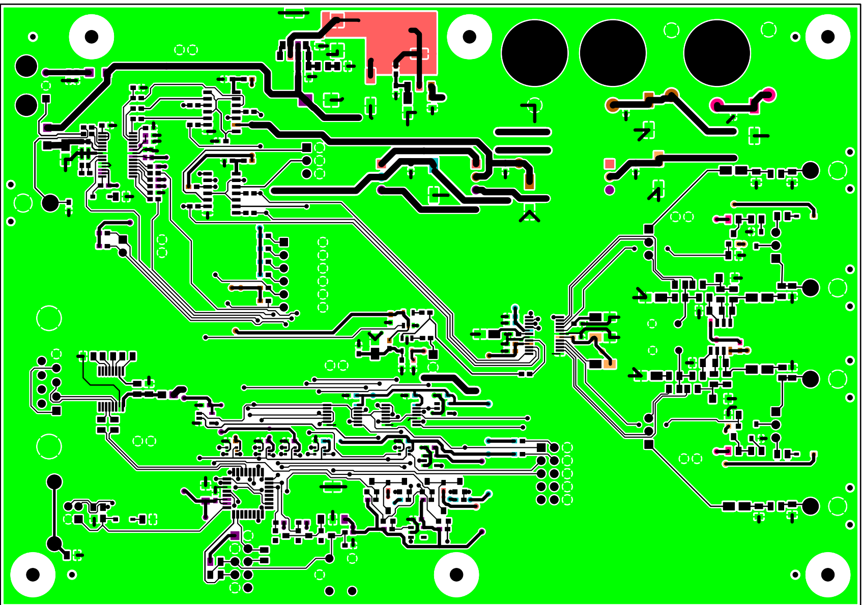
Figure 9. Top Side
