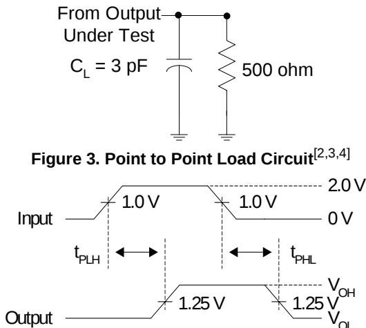
Figure 4. Voltage Waveforms–Propagation Delay Times [3]
