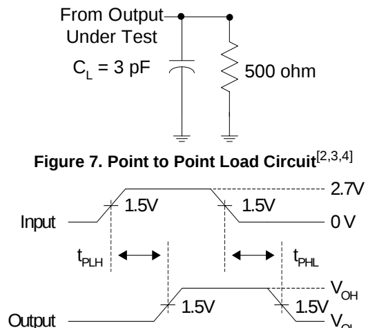
Figure 8. Voltage Waveforms–Propagation Delay Times [3]
