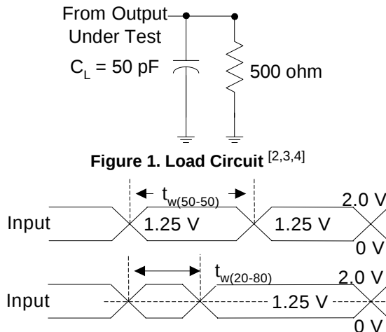
Figure 2. Voltage Waveforms–Pulse Duration [5]
