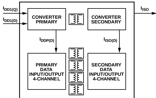
Figure 25. Power Consumption Within the ADuM5401W/ADuM5402W/ADuM5403W
