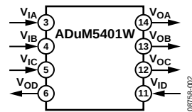
Figure 2. ADuM5401W
