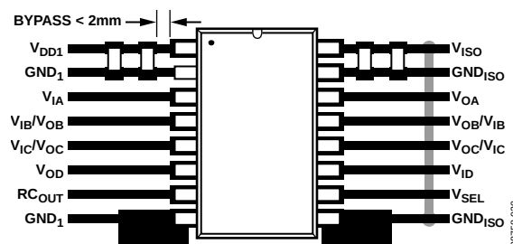
Figure 21. Recommended Printed Circuit Board Layout
