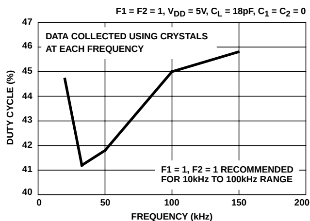
FIGURE 28. DUTY CYCLE vs FREQUENCY
