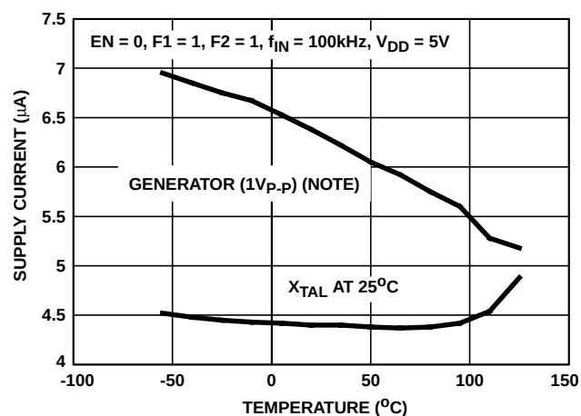
FIGURE 10. DISABLE SUPPLY CURRENT vs TEMPERATURE
