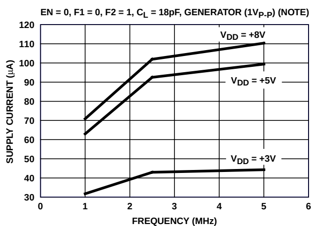
FIGURE 16. DISABLE SUPPLY CURRENT vs FREQUENCY
