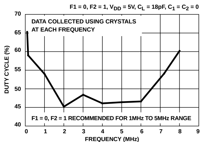
FIGURE 26. DUTY CYCLE vs FREQUENCY
