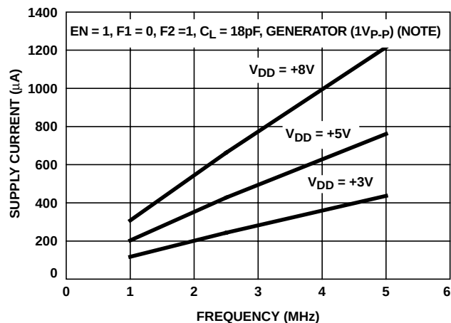
FIGURE 12. SUPPLY CURRENT vs FREQUENCY
