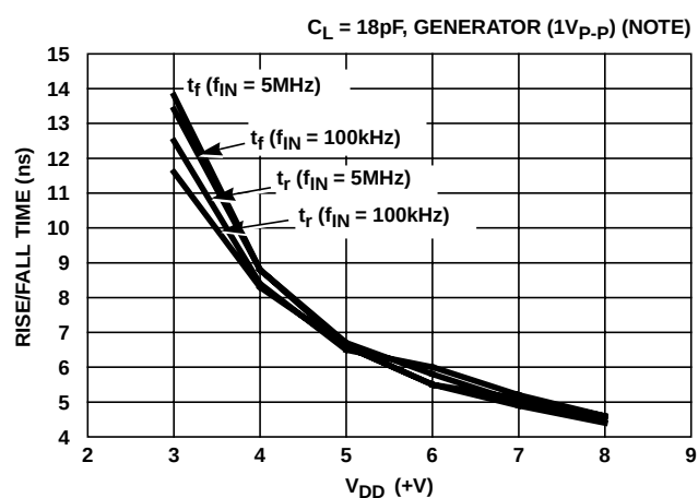
FIGURE 34. RISE/FALL TIME vs V_{DD}
