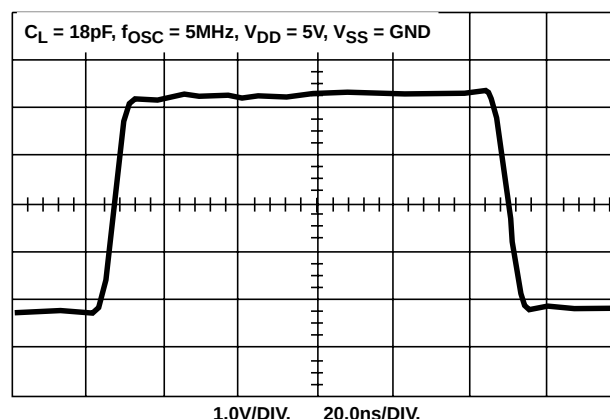
FIGURE 6. OUTPUT WAVEFORM ( C_L = 18\text{pF} )
