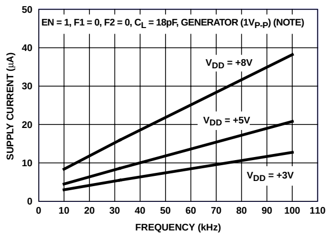
FIGURE 14. SUPPLY CURRENT vs FREQUENCY
