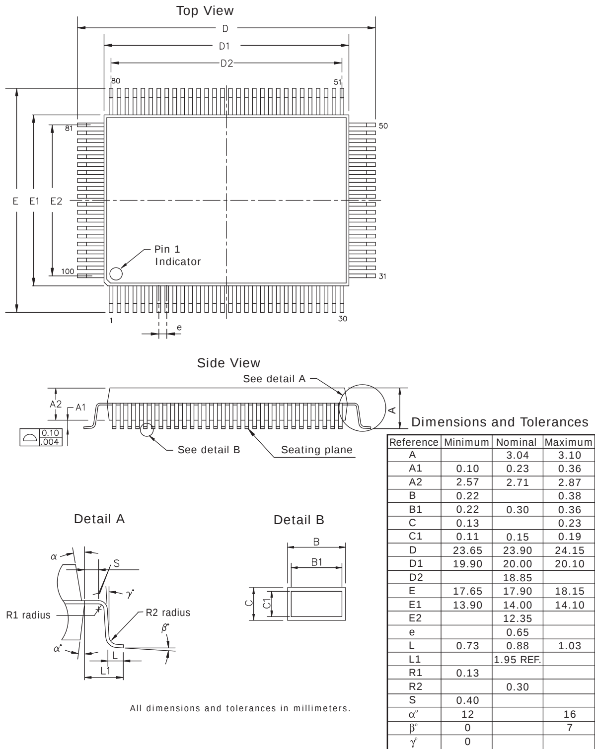
Figure 12. Package Drawing
