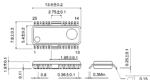
HSOP25
