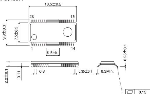
HSOP28
