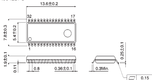
BA6842BFS
