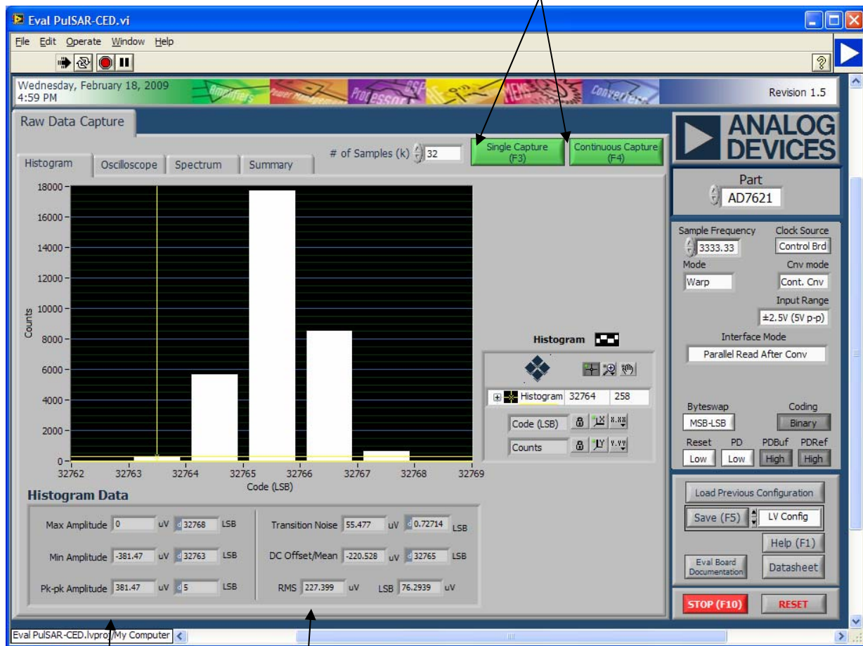
Figure 4. Histogram Screen
