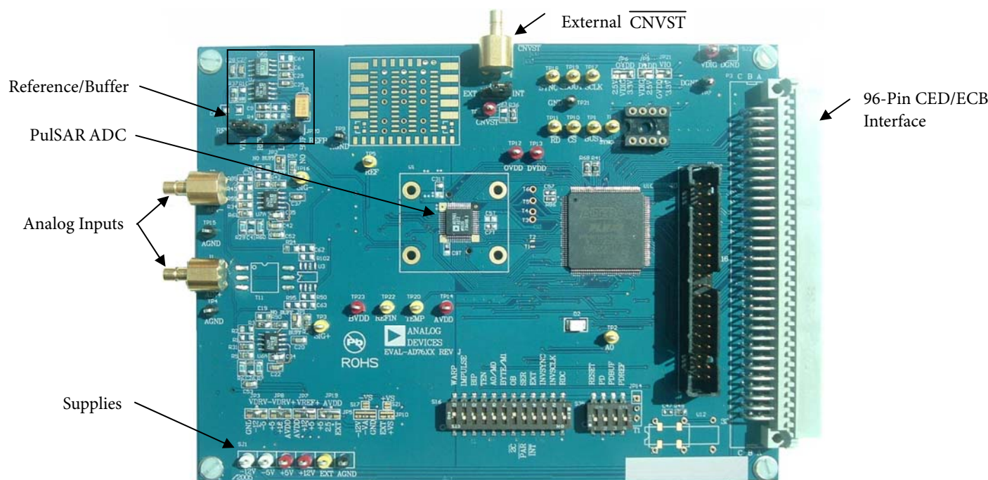
Figure 1. Evaluation Board
