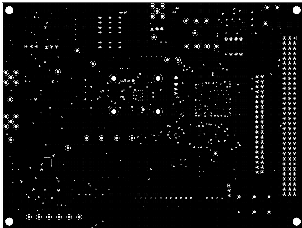
Figure 13. Ground Layer
